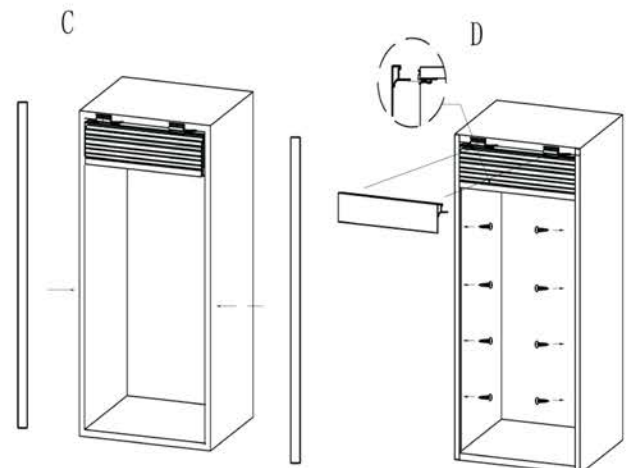
Installation of baffle board and tracks
